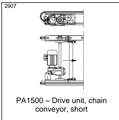
PA1500 – Drive unit chain conveyor for small c/c between chain strings
