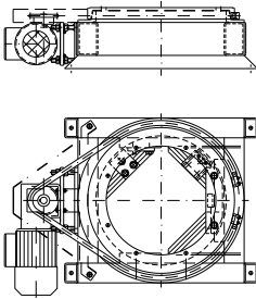
AX100 – Vridmodul, driven
